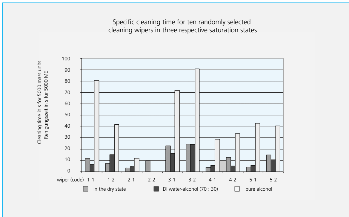
Fig. 19 Diagram: Specific cleaning time for ten randomly selected cleaning wipers in three respective saturation states
