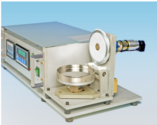
Fig. 6 Test device Labuda Rotation Wiping Simulator Mark II
