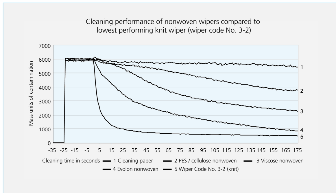
Fig.14 Diagram: Cleaning performance of nonwoven wipers compared to a knit wiper
