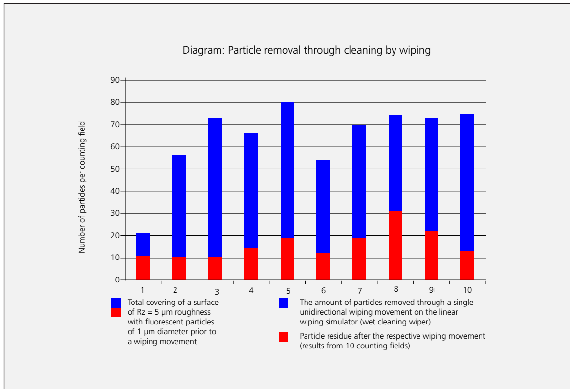
Fig.15 Diagram: Particle removal through cleaning by wiping
