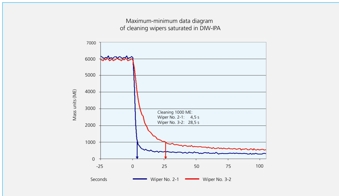
Fig. 11 Diagram: Comparison of the wiper with the highest and with the lowest specific cleaning time
