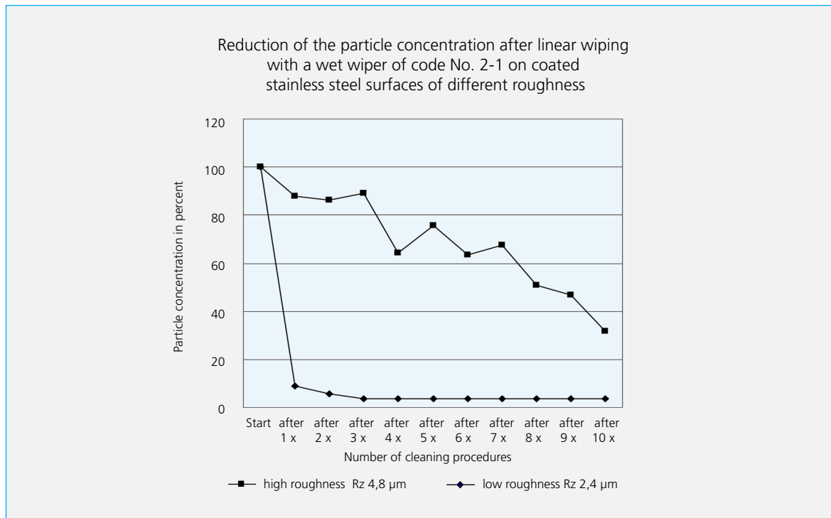
Fig.18 Diagram: Reduction of the particle concentration after linear wiping with a wet wiper of code No. 2-1
