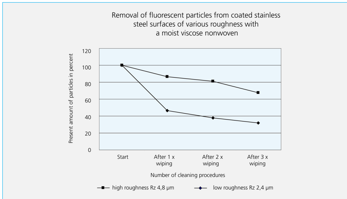
Fig.13 Diagram: Removal of fluorescent particles from coated stainless steel surfaces of various roughness with a moist viscose nonwoven
