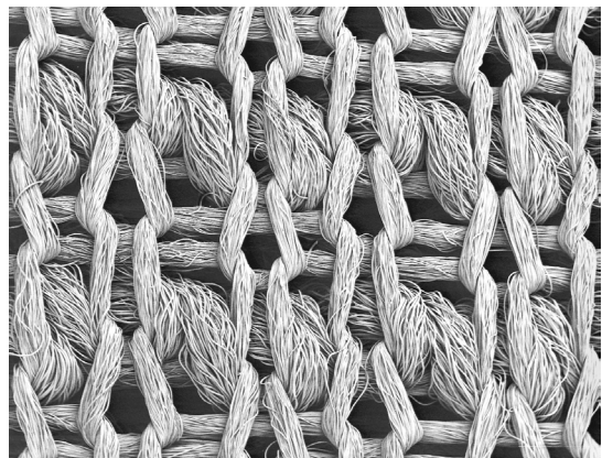
Fig. 3 Coarse knit Sibis GD-U
