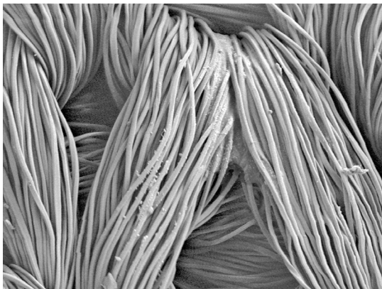
Fig. 16 SEM photo of a knit wiper after completed cleaning procedure. In the middle strand of yarn you can clearly see the accumulated particles.
