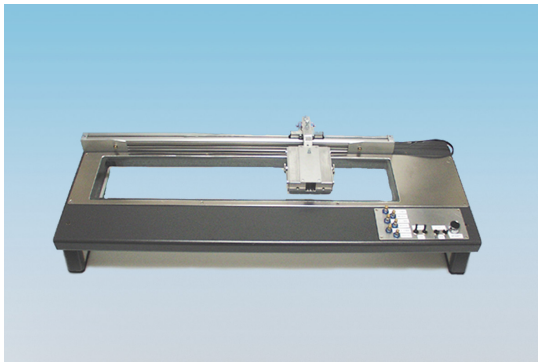
Fig. 5 Test device Labuda Linear Wiping Simulator Mark II
