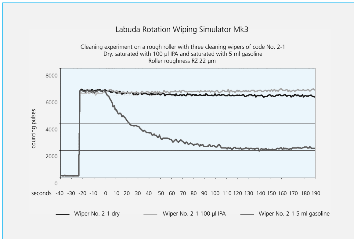
Fig. 23 Diagram: Different cleaning performances of the same knit wiper with a rough surface (RZ 22 µm) and varying kinds of solvents
