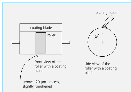
Fig. 7 Schematic diagram of the cleaning time test device Labuda Rotation Wiping Simulator Mk III
